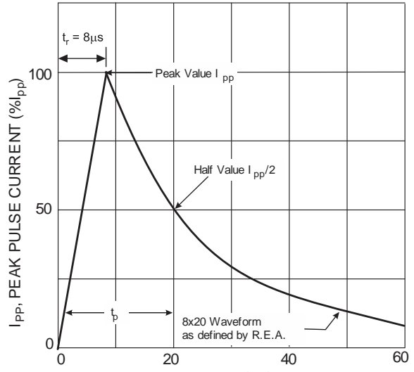
Figure 8 Pulse Waveform
